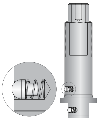
Anti-static design
