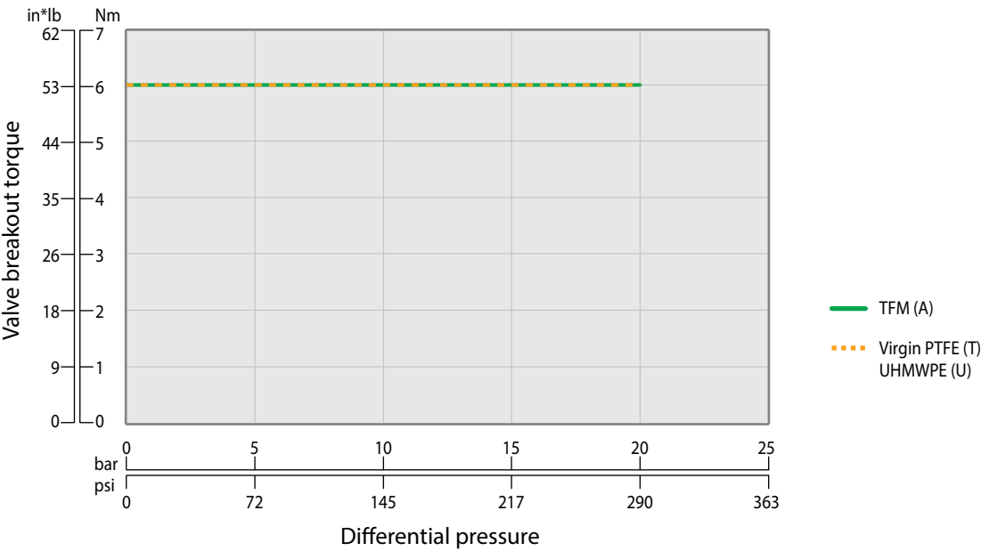
Pressure class: #300 | Full port: 1/2" (DN15) | 48 Series
