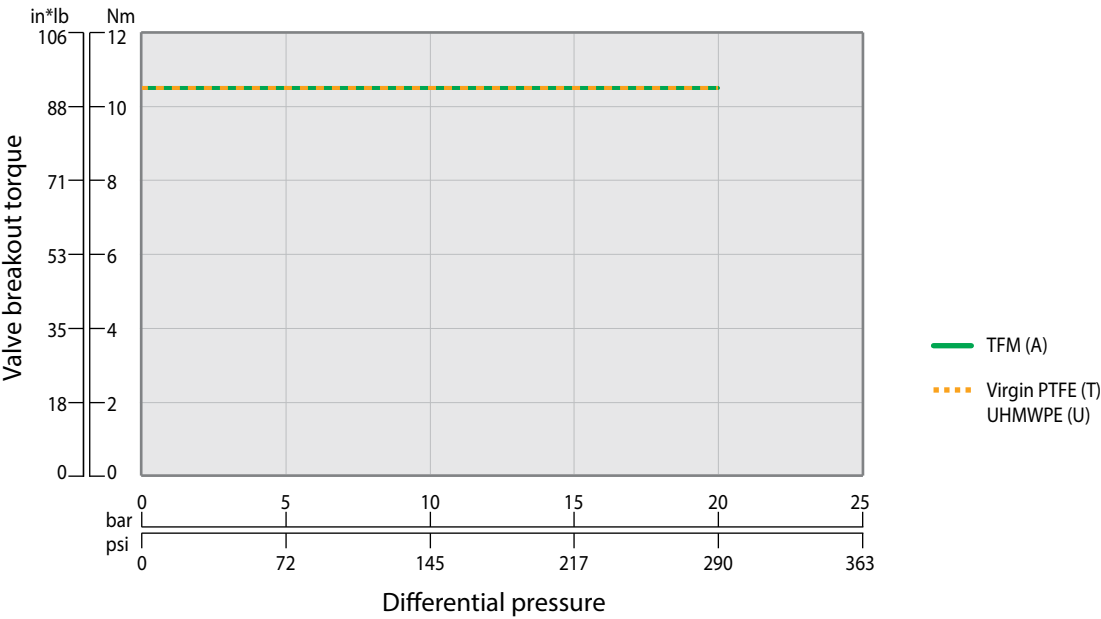
Pressure class: #300 | Full port: 3/4" (DN20) | 48 Series
