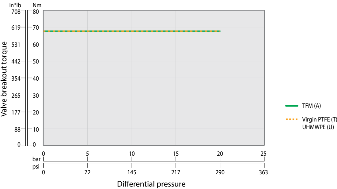
Pressure class: #300 | Full port: 2" (DN50) | 48 Series
