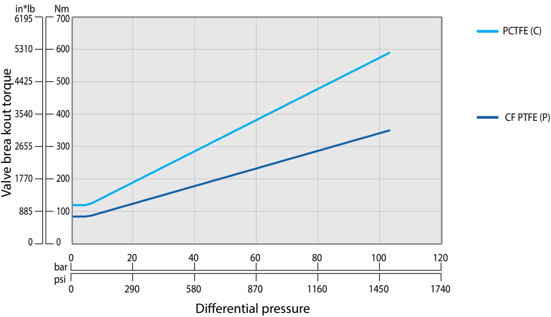
Pressure class: #600 | Full port: 2" (DN50) | C26 Series
