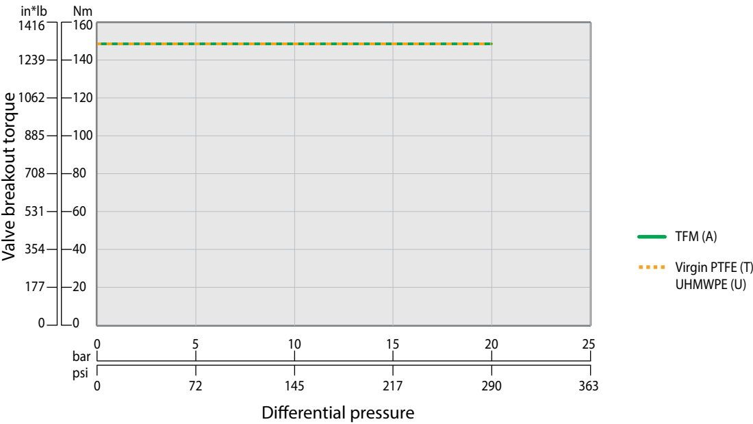
Pressure class: #300 | Full port: 3" (DN80) | 48 Series
