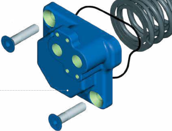
Spring cartridge: Improves the torque characteristics of the CompAct actuator
