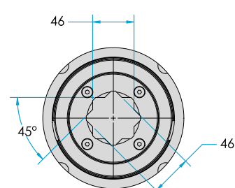
DETAIL F OPTIONAL ADAPTER ISO 5211 46mm SQUARE SHAFT INSERT MAX 4000Nm
